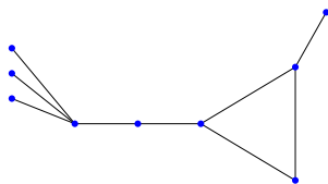
Figure 1: A compressible graph in \mathbb{R}^1 .
