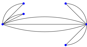
Figure 3: A compressed generic realization of a graph with two cut-vertices.
