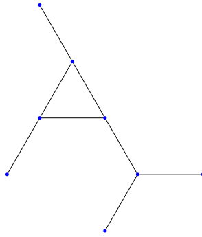
Figure 2: A graph which is not compressible in \mathbb{R}^1 .
