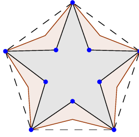
Figure 4: A compressed two-dimensional realization of graph G . The dashed edges represent \bar{G} .
